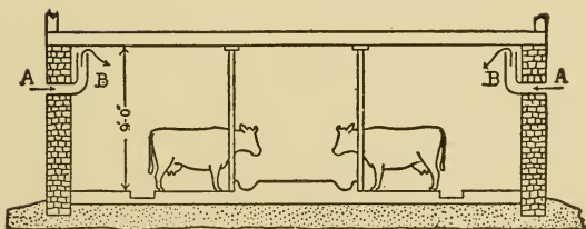
Sketch A—Two methods of ventilating a dairy barn.
